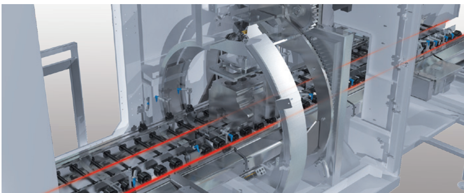
Emptying station to pivot the block
