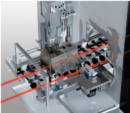
Pre-control unit
