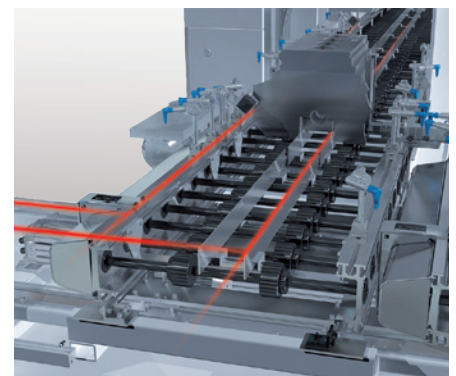
SPC Shuttle for sampling
